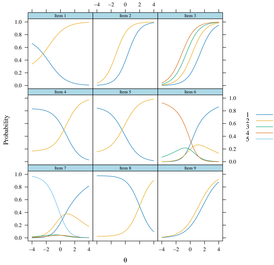
Figure 1: Item response curves.
